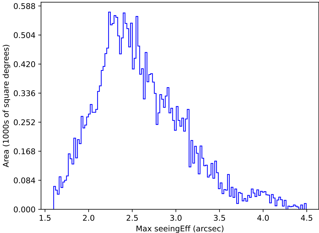
ddf_loaded_half_fl4_v3.4_10yrs All sky r band: Max seeingEff
