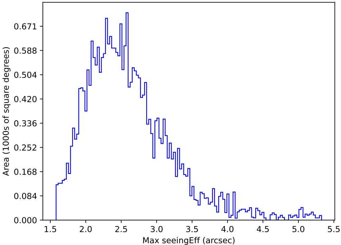
ddf_loaded_half_fl4_v3.4_10yrs All sky i band: Max seeingEff
