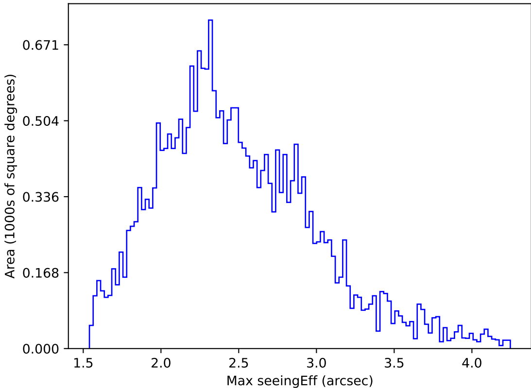
ddf_loaded_half_fl4_v3.4_10yrs All sky g band: Max seeingEff
