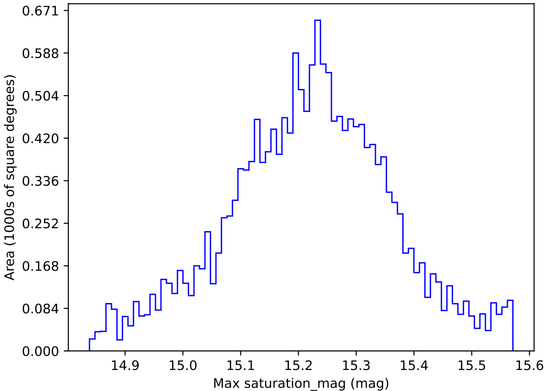
ddf_loaded_half_fl4_v3.4_10yrs WFD z band: Max saturation_mag
