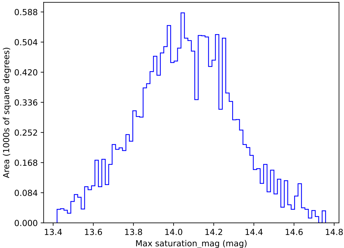
ddf_loaded_half_fl4_v3.4_10yrs WFD u band: Max saturation_mag
