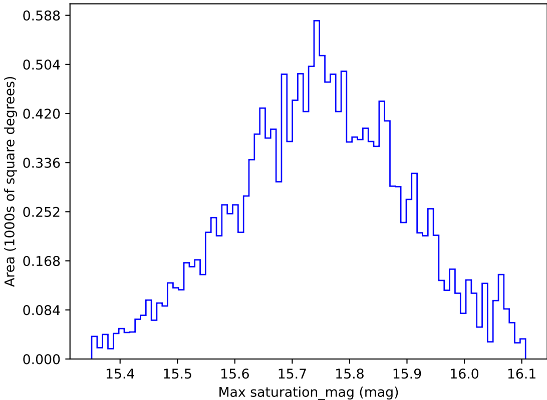
ddf_loaded_half_fl4_v3.4_10yrs WFD r band: Max saturation_mag
