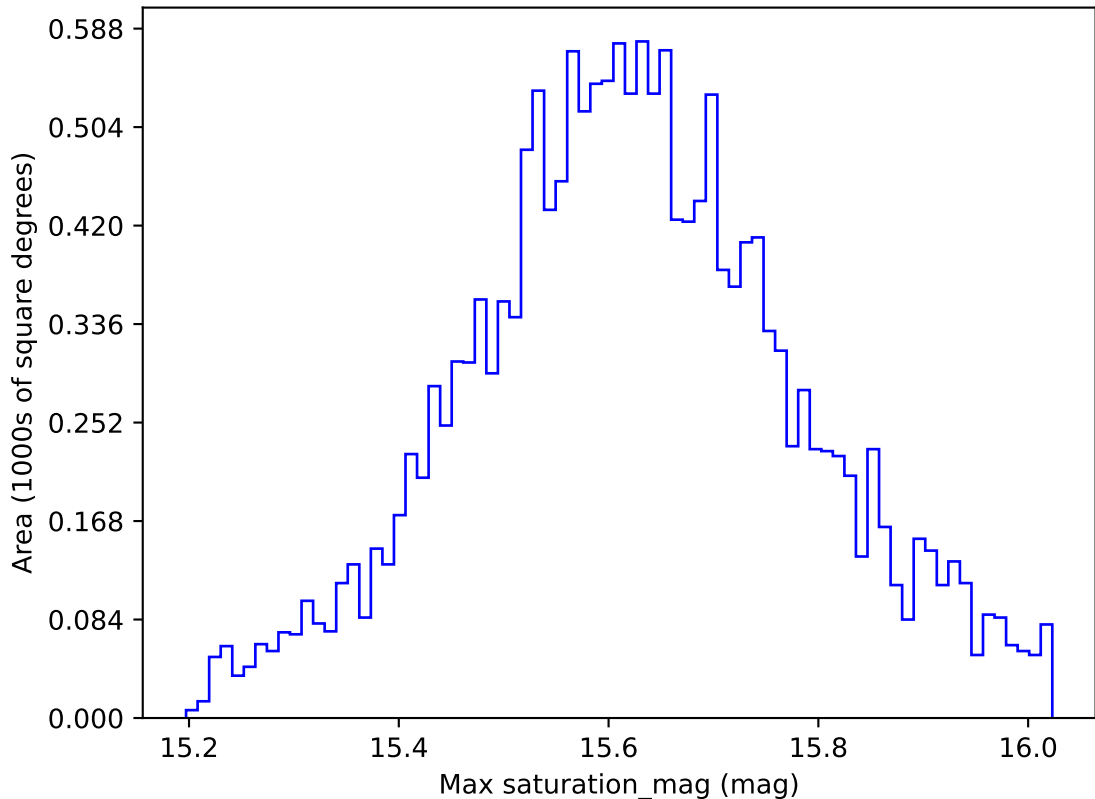
ddf_loaded_half_fl4_v3.4_10yrs WFD i band: Max saturation_mag
