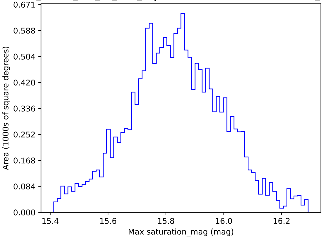
ddf_loaded_half_f14_v3.4_10yrs WFD all bands: Max saturation_mag
