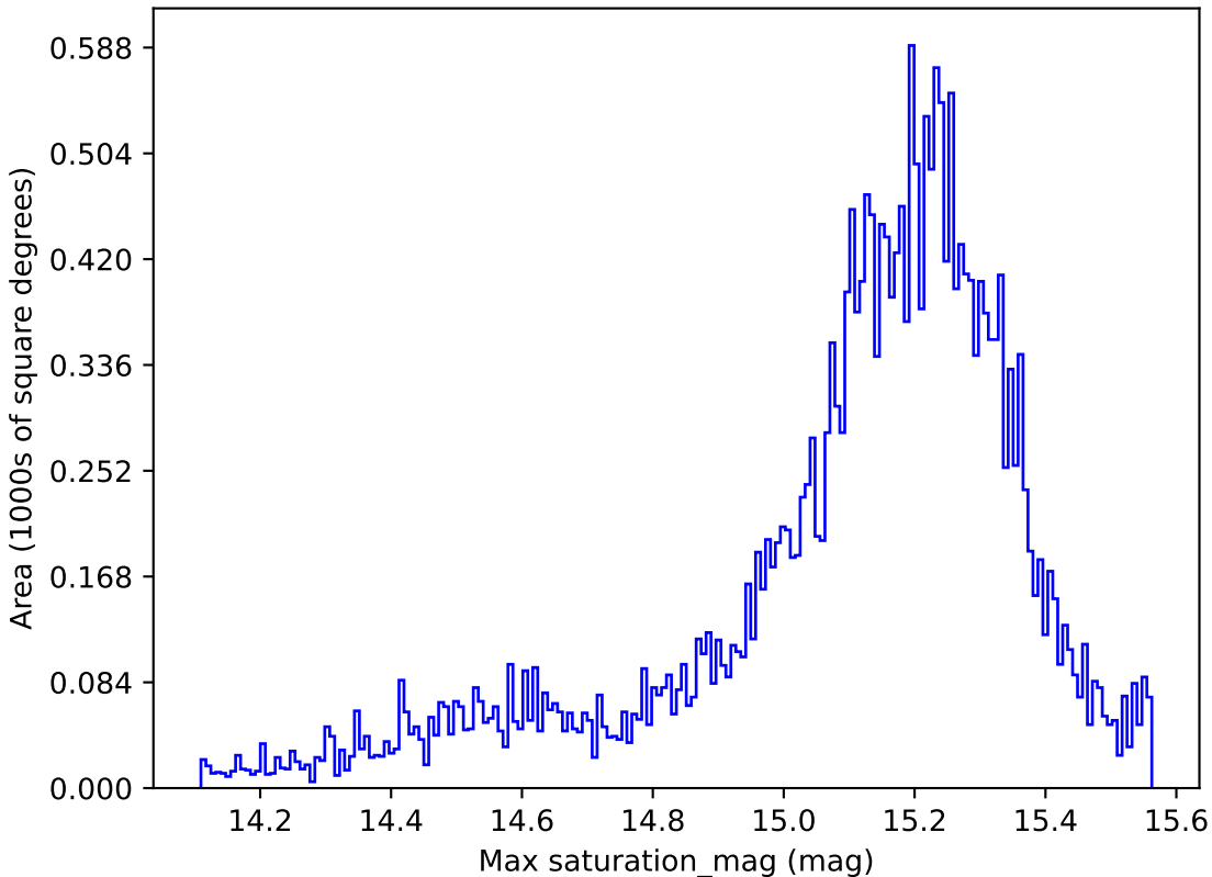
ddf_loaded_half_fl4_v3.4_10yrs All sky z band: Max saturation_mag
