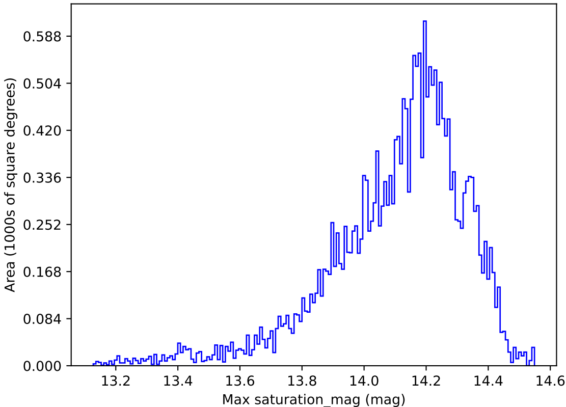
ddf_loaded_half_fl4_v3.4_10yrs All sky y band: Max saturation_mag
