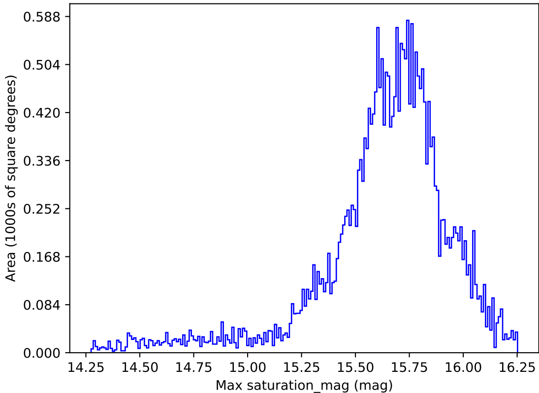
ddf_loaded_half_fl4_v3.4_10yrs All sky g band: Max saturation_mag
