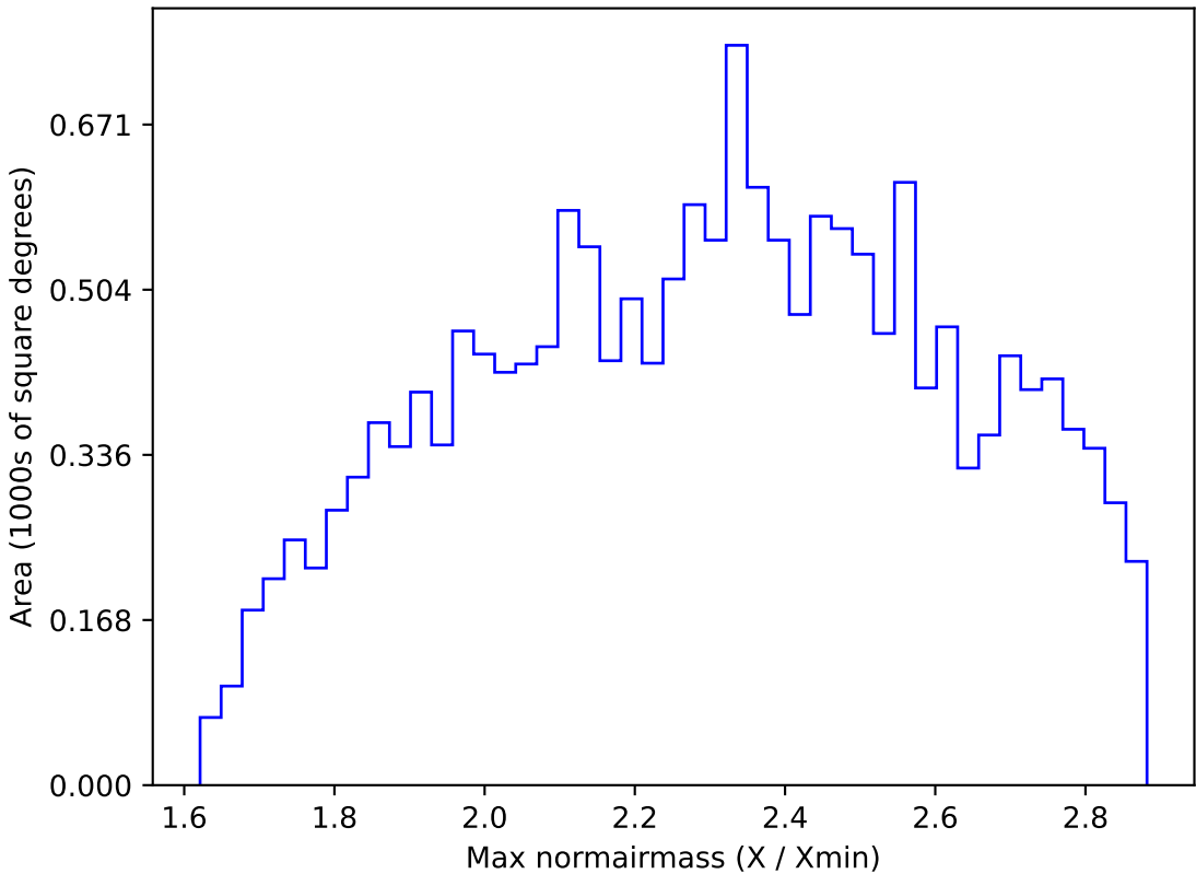
ddf_loaded_half_fl4_v3.4_10yrs WFD z band: Max normairmass
