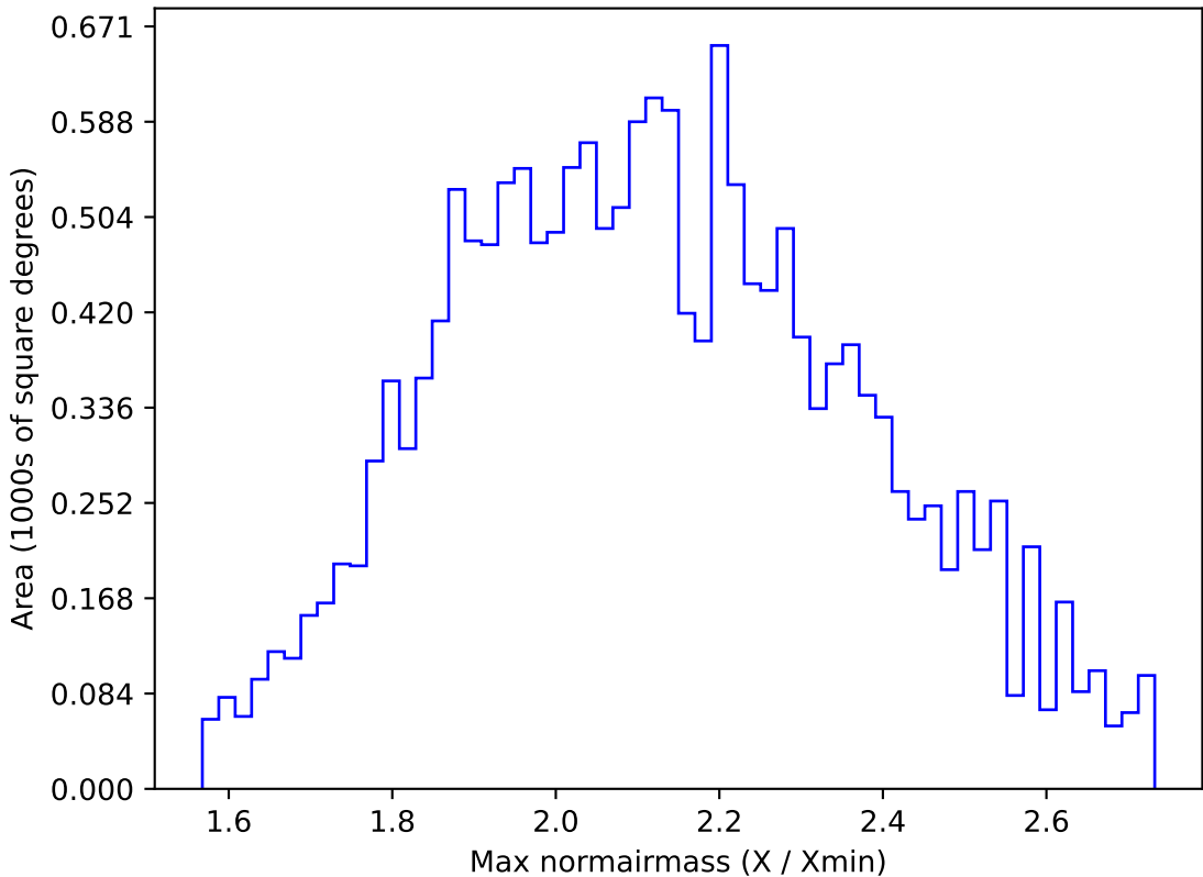
ddf_loaded_half_fl4_v3.4_10yrs WFD y band: Max normairmass
