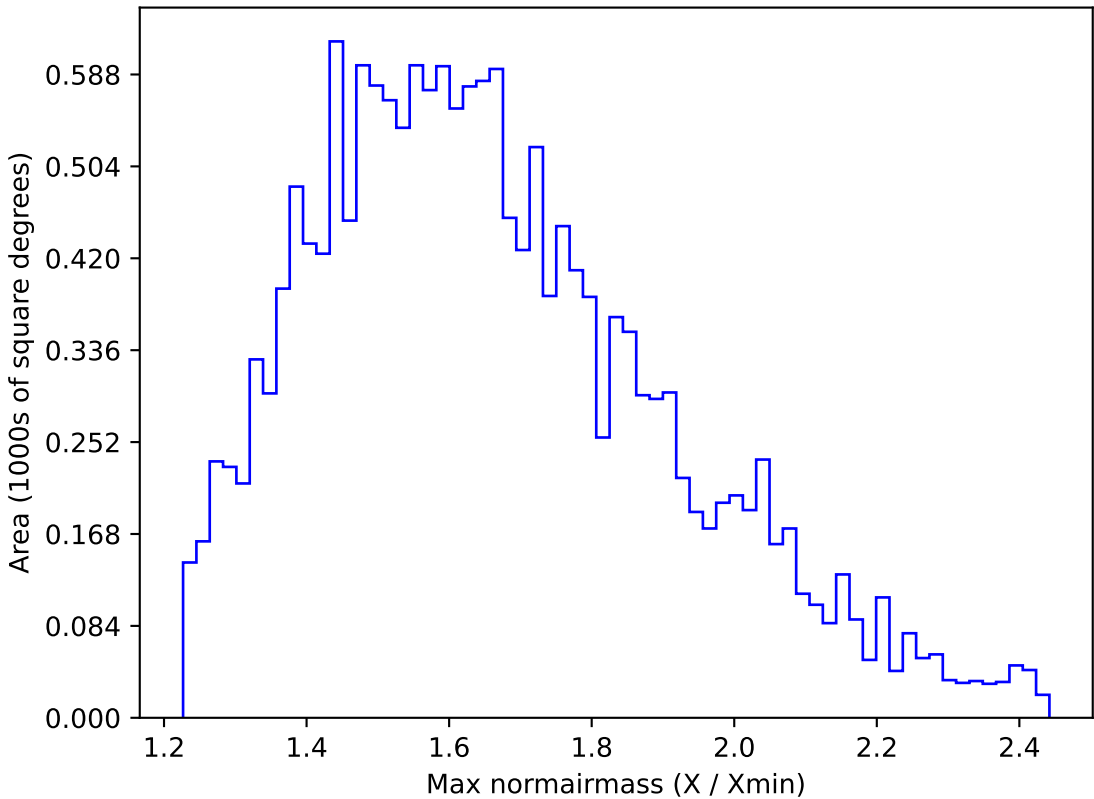
ddf_loaded_half_fl4_v3.4_10yrs WFD u band: Max normairmass
