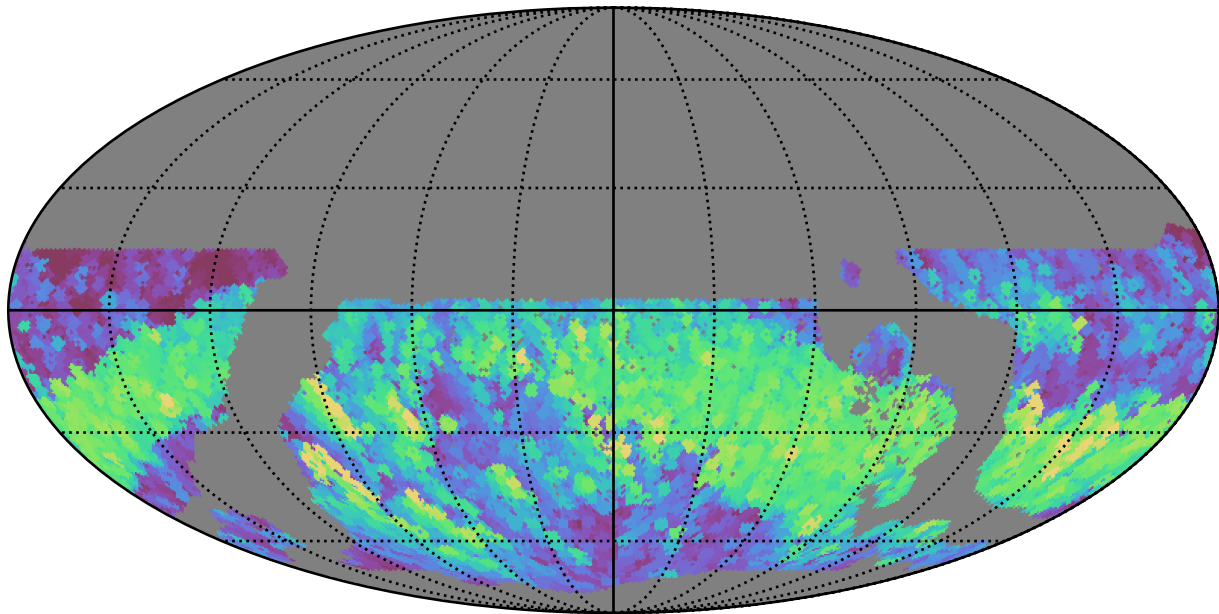
ddf_loaded_half_fl4_v3.4_10yrs WFD r band: Max normairmass
