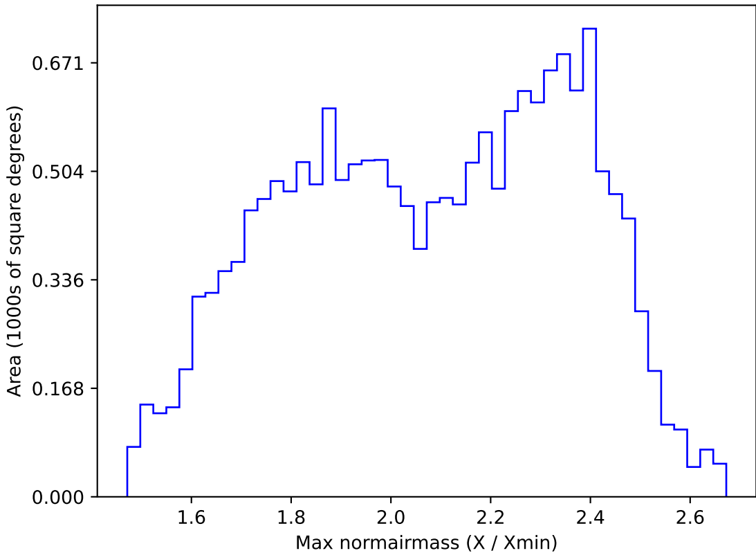
ddf_loaded_half_fl4_v3.4_10yrs WFD r band: Max normairmass
