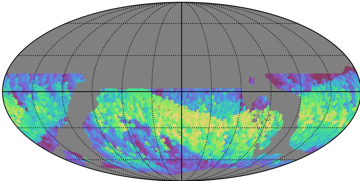
ddf_loaded_half_fl4_v3.4_10yrs WFD i band: Max normairmass
