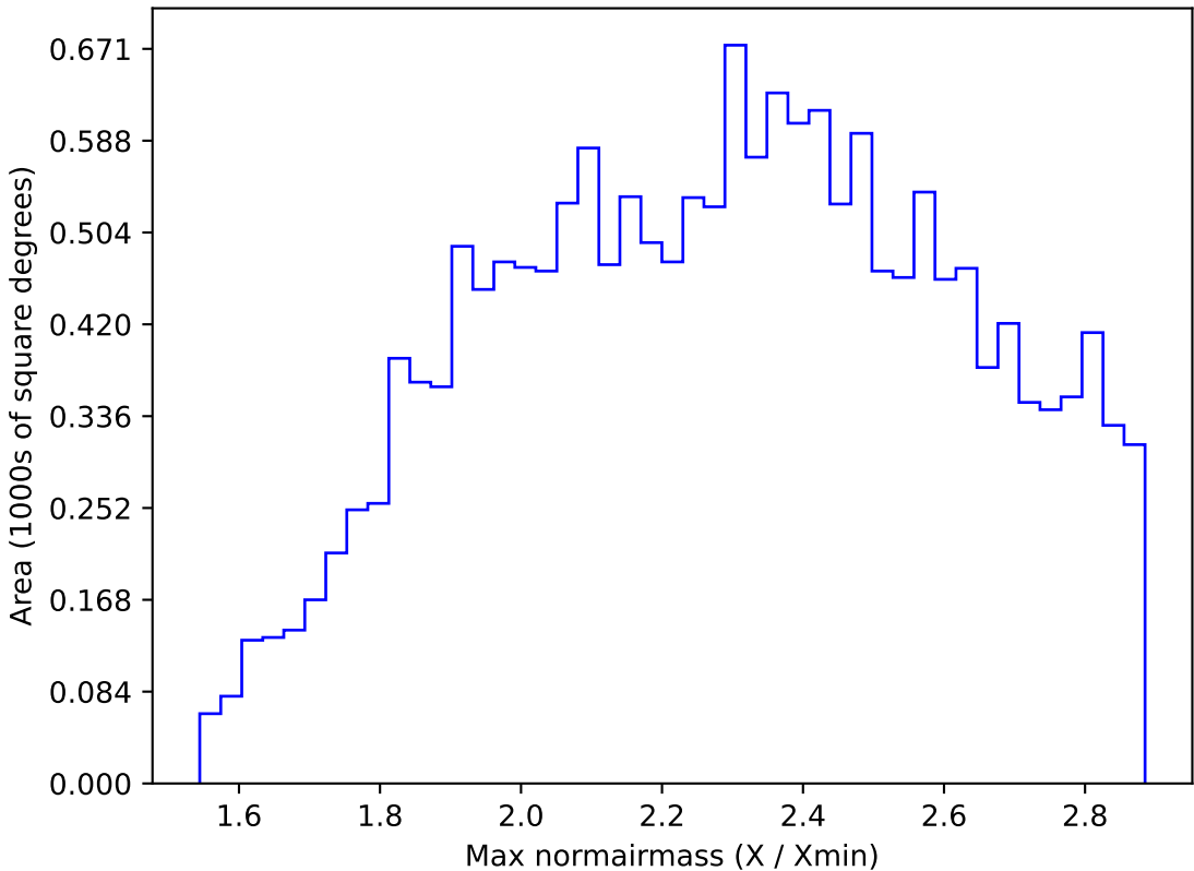
ddf_loaded_half_fl4_v3.4_10yrs WFD i band: Max normairmass
