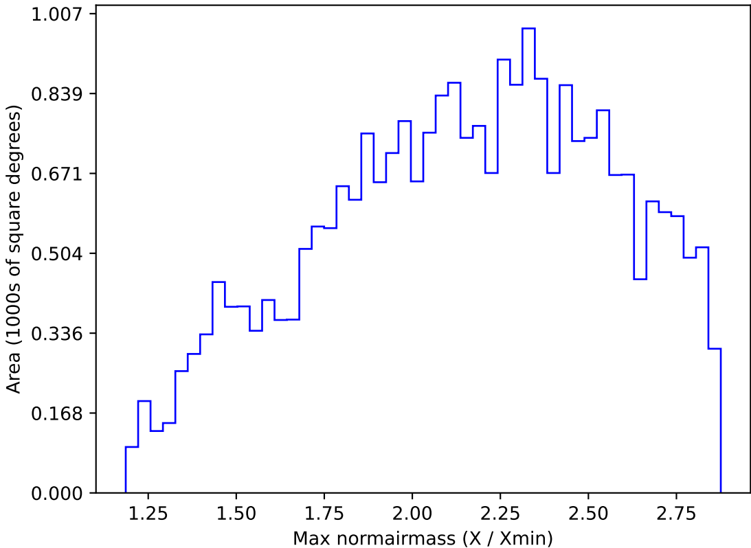
ddf_loaded_half_fl4_v3.4_10yrs All sky z band: Max normairmass
