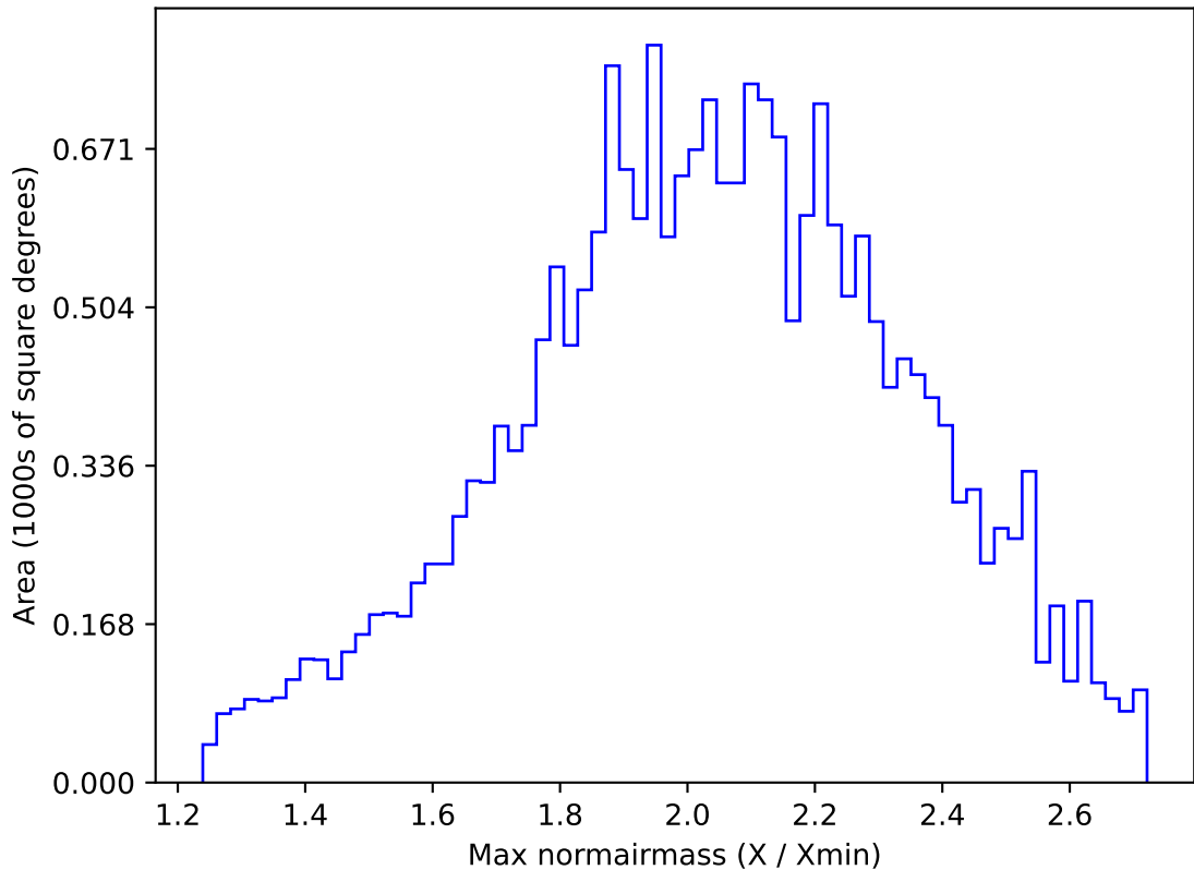
ddf_loaded_half_fl4_v3.4_10yrs All sky y band: Max normairmass
