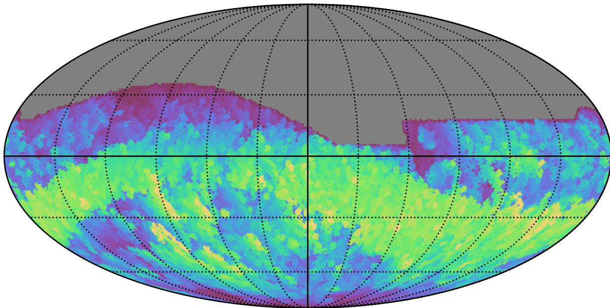
ddf_loaded_half_fl4_v3.4_10yrs All sky r band: Max normairmass
