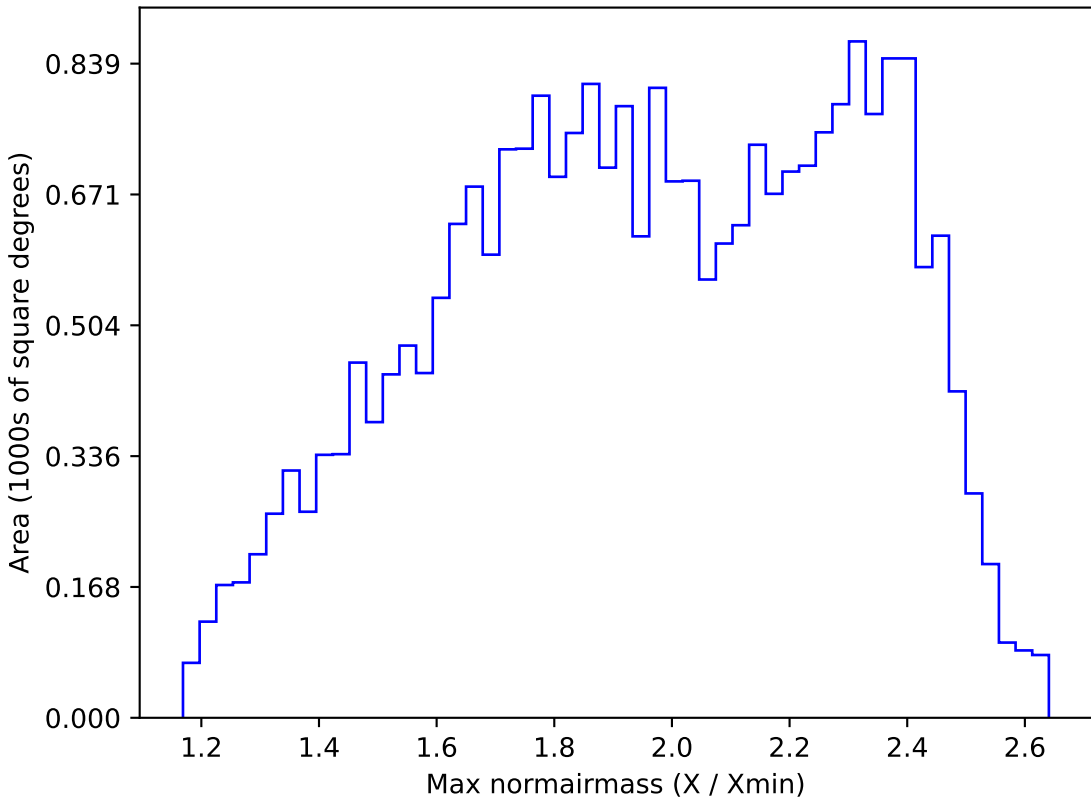
ddf_loaded_half_fl4_v3.4_10yrs All sky r band: Max normairmass
