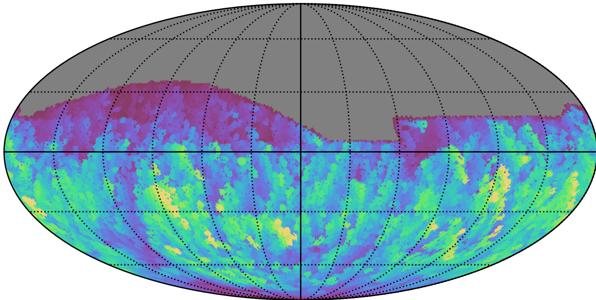
ddf_loaded_half_fl4_v3.4_10yrs All sky g band: Max normairmass
