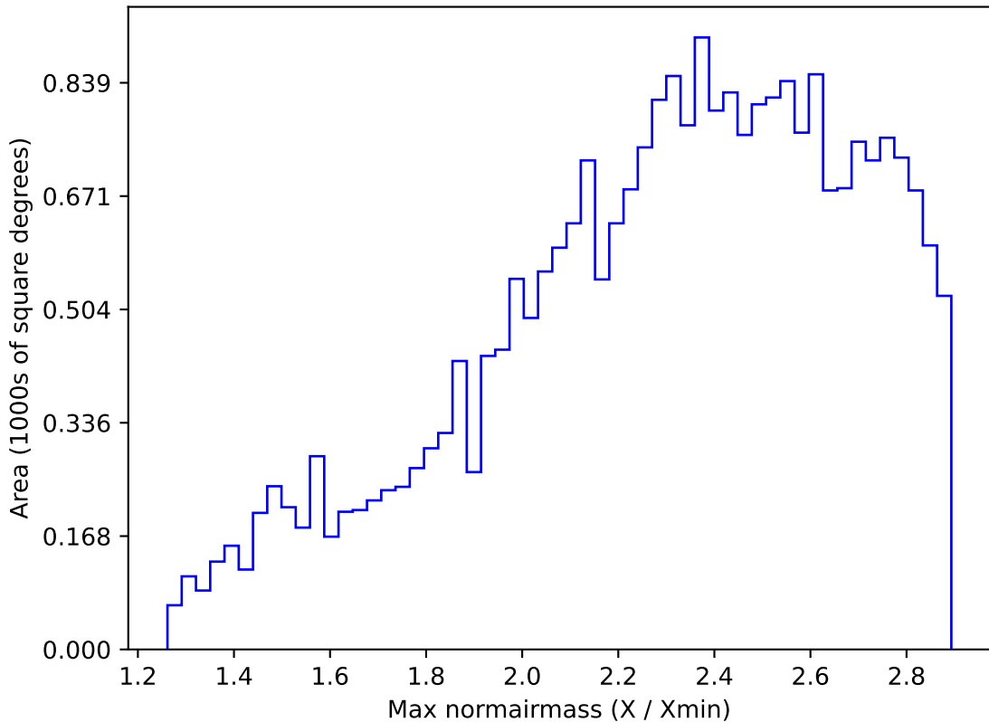
ddf_loaded_half_fl4_v3.4_10yrs All sky all bands: Max normairmass
