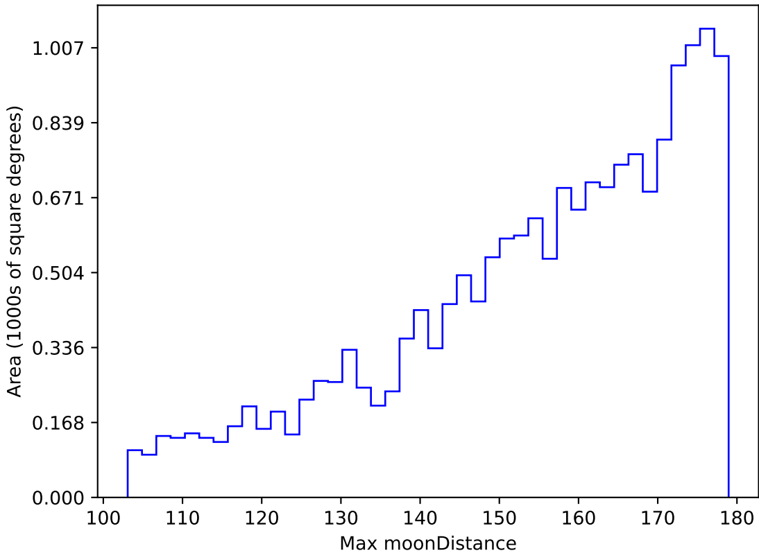
ddf_loaded_half_fl4_v3.4_10yrs WFD z band: Max moonDistance
