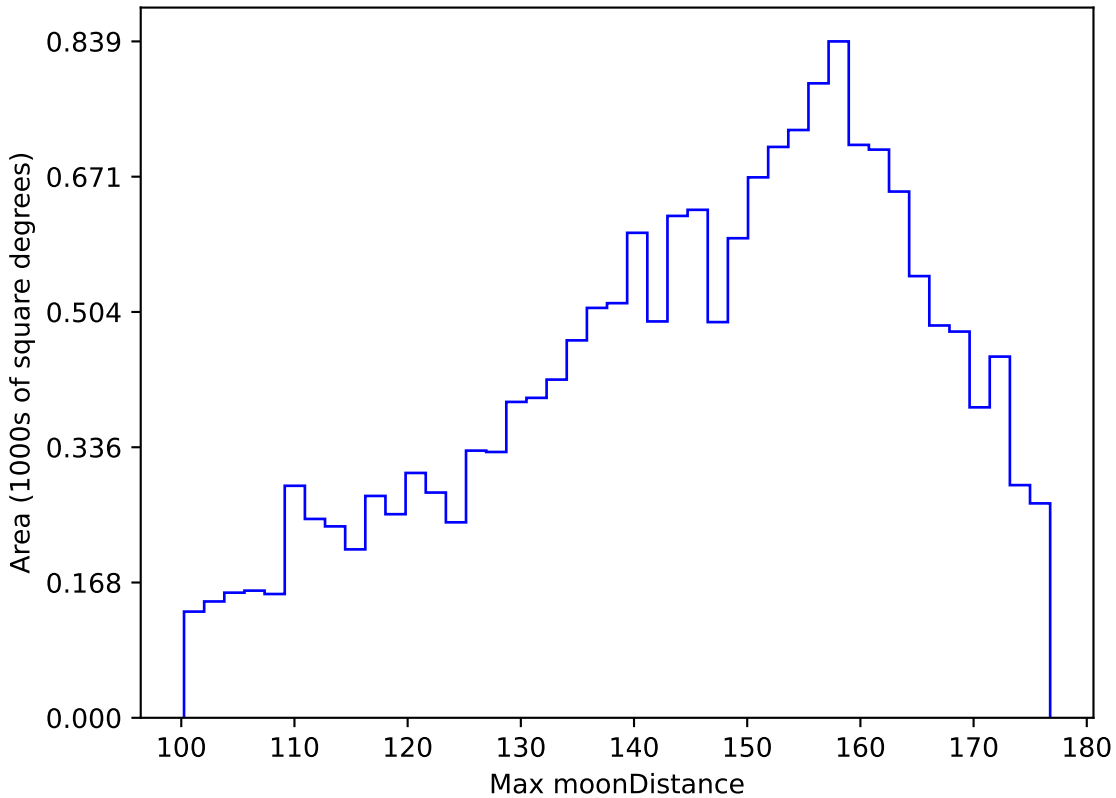
ddf_loaded_half_fl4_v3.4_10yrs WFD y band: Max moonDistance
