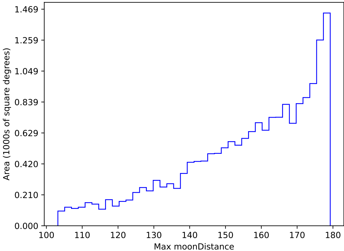
ddf_loaded_half_fl4_v3.4_10yrs WFD i band: Max moonDistance
