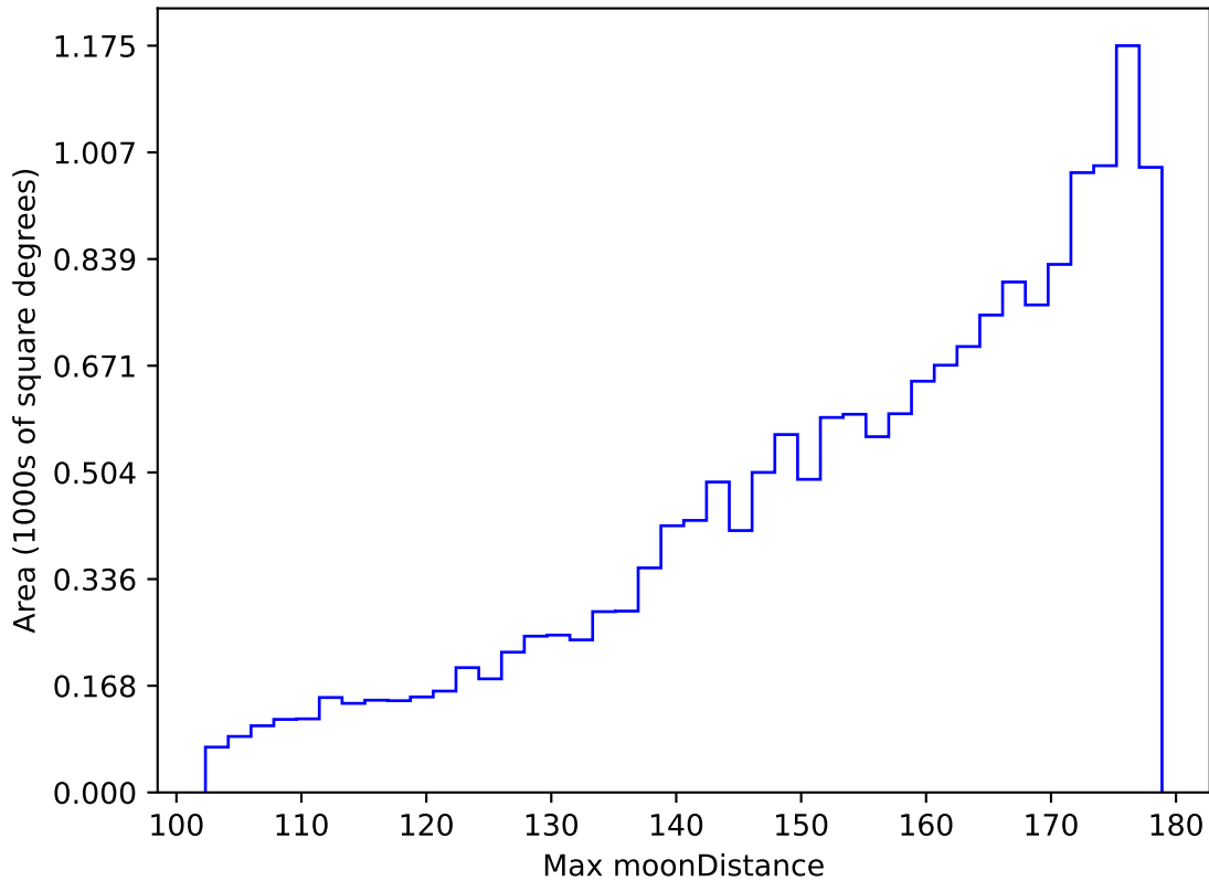
ddf_loaded_half_fl4_v3.4_10yrs WFD g band: Max moonDistance
