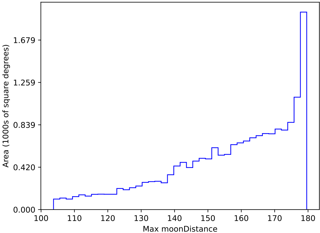
ddf_loaded_half_fl4_v3.4_10yrs WFD all bands: Max moonDistance
