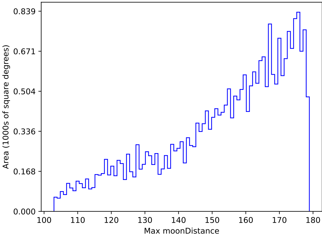
ddf_loaded_half_fl4_v3.4_10yrs All sky z band: Max moonDistance
