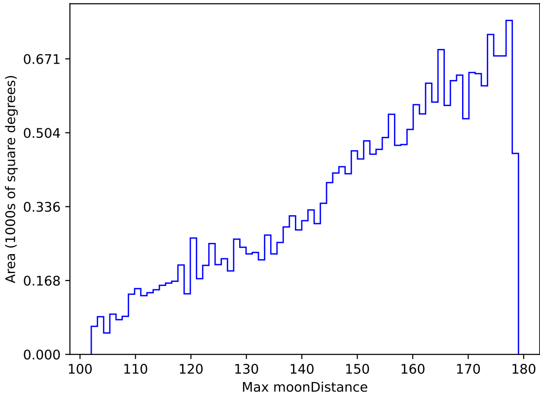
ddf_loaded_half_fl4_v3.4_10yrs All sky u band: Max moonDistance
