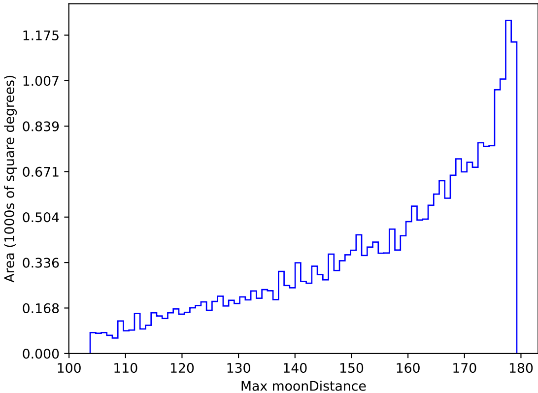
ddf_loaded_half_fl4_v3.4_10yrs All sky r band: Max moonDistance
