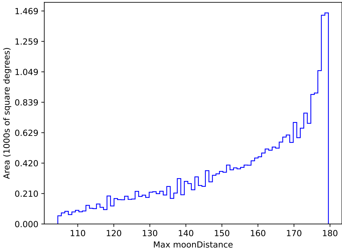
ddf_loaded_half_fl4_v3.4_10yrs All sky all bands: Max moonDistance
