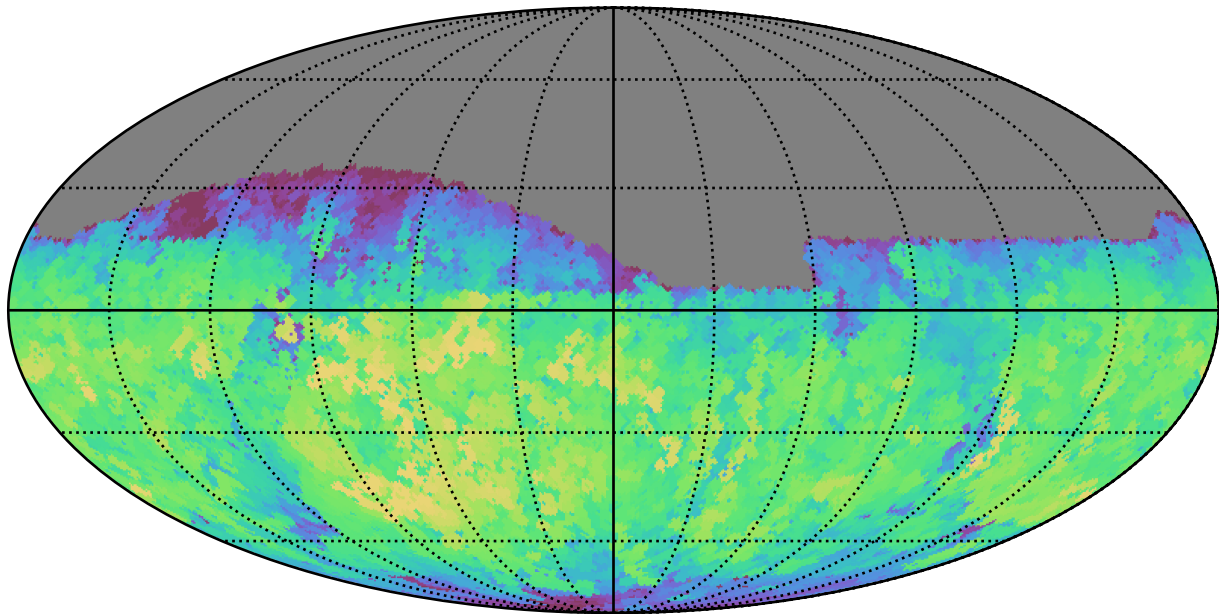
ddf_loaded_half_fl4_v3.4_10yrs Yr 1 z band: Max fiveSigmaDepth
