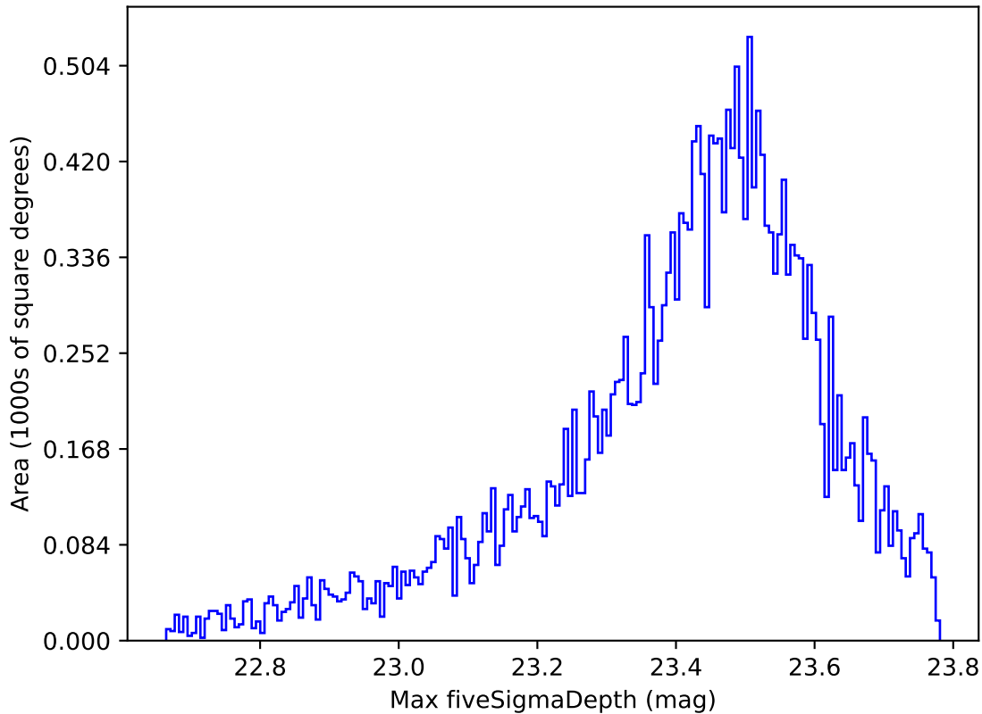
ddf_loaded_half_fl4_v3.4_10yrs Yr 1 z band: Max fiveSigmaDepth
