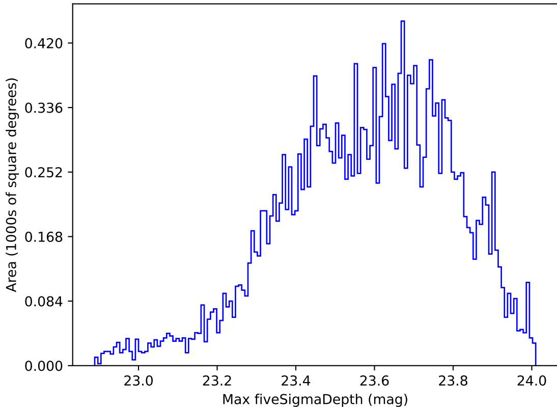
ddf_loaded_half_fl4_v3.4_10yrs Yr 1 u band: Max fiveSigmaDepth
