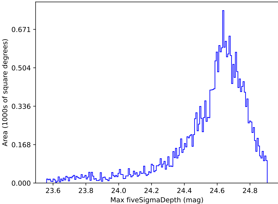
ddf_loaded_half_fl4_v3.4_10yrs Yr 1 r band: Max fiveSigmaDepth
