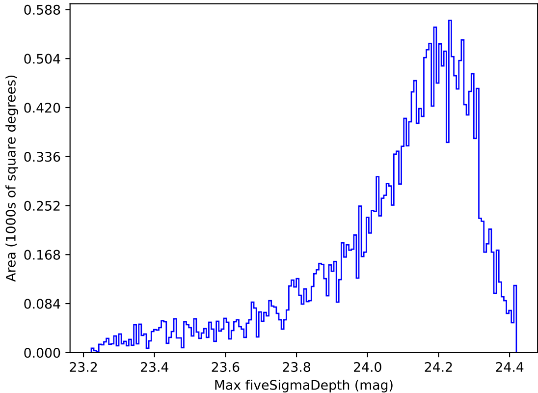
ddf_loaded_half_fl4_v3.4_10yrs Yr 1 i band: Max fiveSigmaDepth
