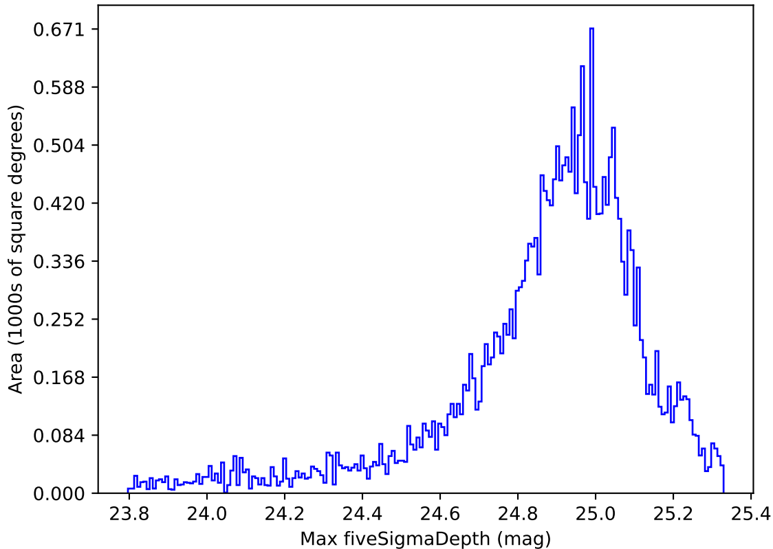
ddf_loaded_half_fl4_v3.4_10yrs Yr 1 g band: Max fiveSigmaDepth
