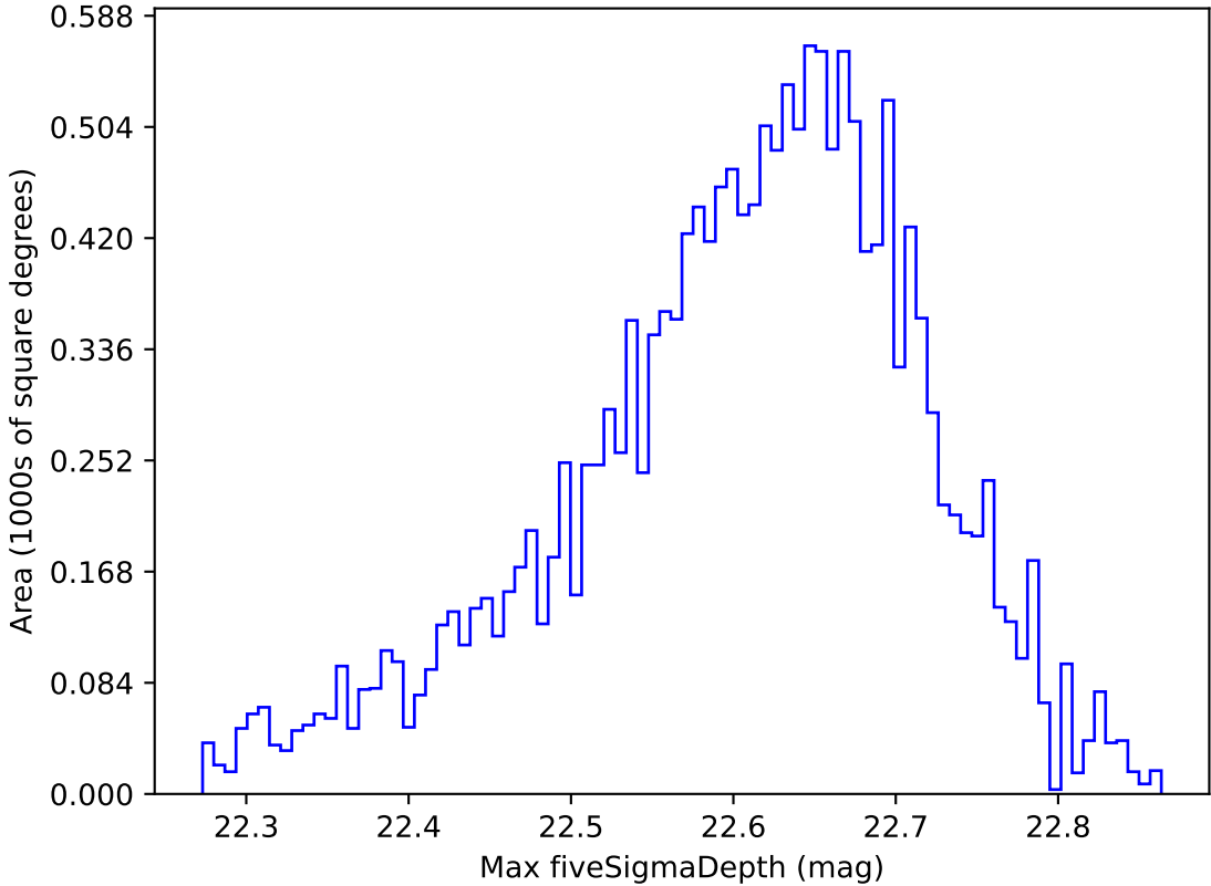
ddf_loaded_half_fl4_v3.4_10yrs WFD y band: Max fiveSigmaDepth
