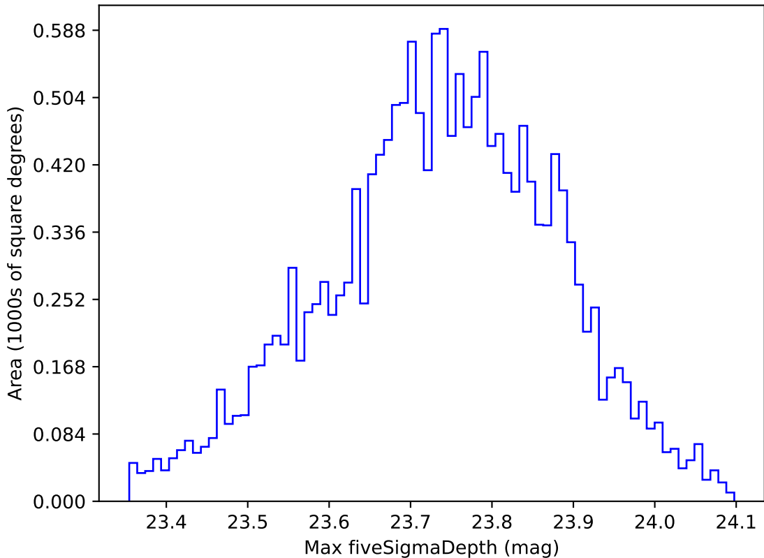
ddf_loaded_half_fl4_v3.4_10yrs WFD u band: Max fiveSigmaDepth
