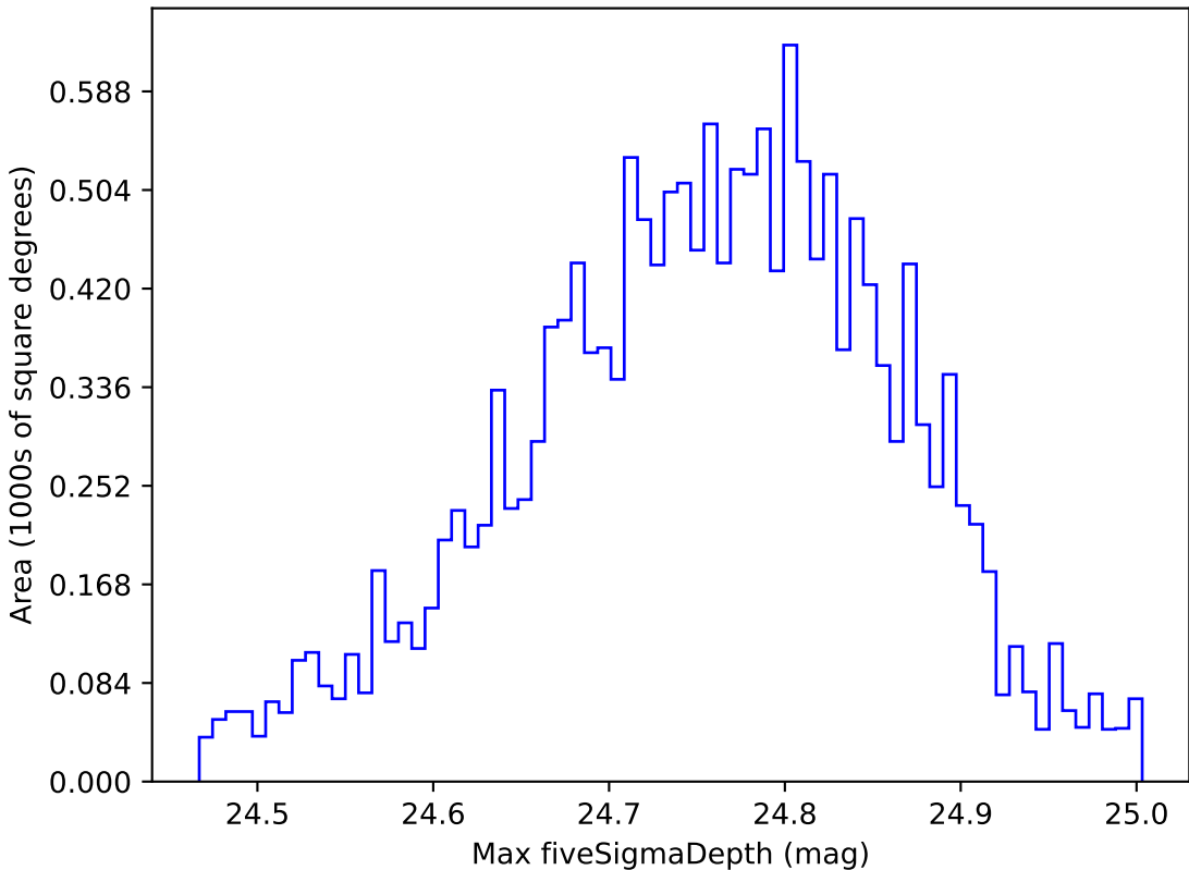
ddf_loaded_half_fl4_v3.4_10yrs WFD r band: Max fiveSigmaDepth
