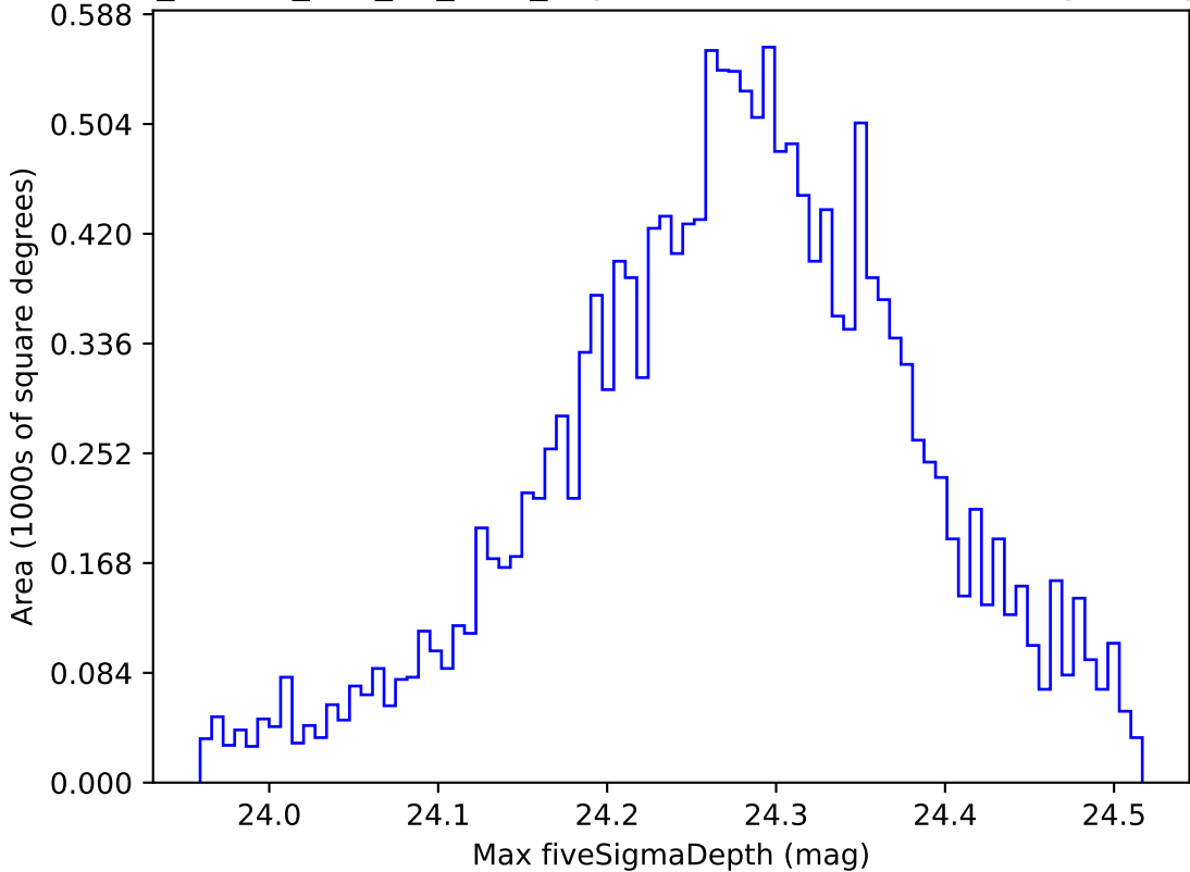
ddf_loaded_half_fl4_v3.4_10yrs WFD i band: Max fiveSigmaDepth
