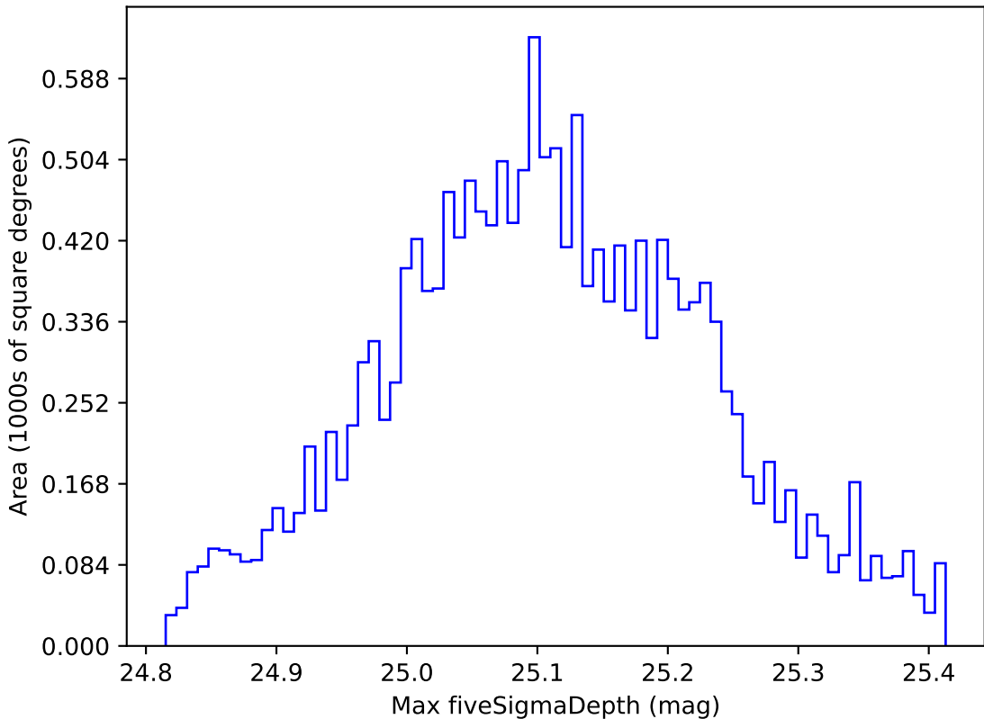
ddf_loaded_half_fl4_v3.4_10yrs WFD g band: Max fiveSigmaDepth
