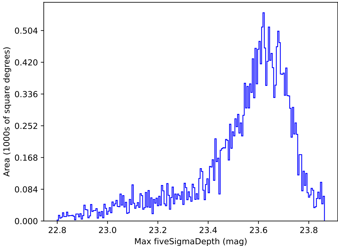
ddf_loaded_half_fl4_v3.4_10yrs All sky z band: Max fiveSigmaDepth
