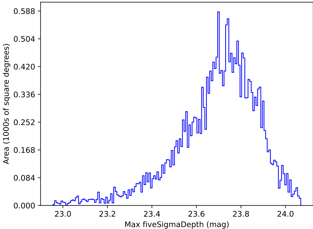
ddf_loaded_half_fl4_v3.4_10yrs All sky u band: Max fiveSigmaDepth
