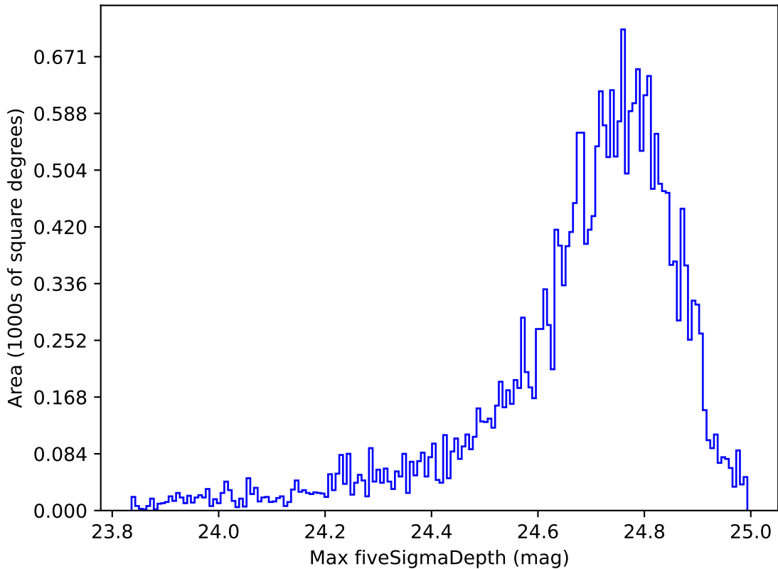
ddf_loaded_half_fl4_v3.4_10yrs All sky r band: Max fiveSigmaDepth
