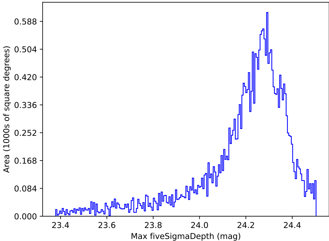
ddf_loaded_half_fl4_v3.4_10yrs All sky i band: Max fiveSigmaDepth
