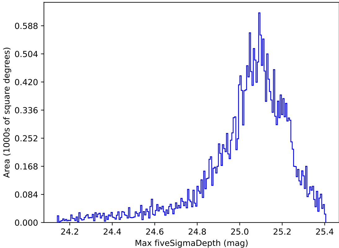
ddf_loaded_half_fl4_v3.4_10yrs All sky g band: Max fiveSigmaDepth
