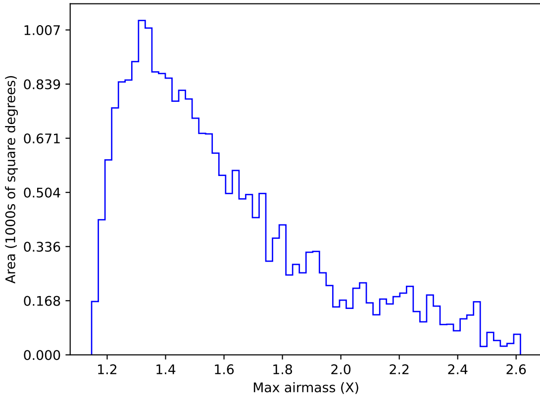
ddf_loaded_half_f14_v3.4_10yrs Yr 1 y band: Max airmass
